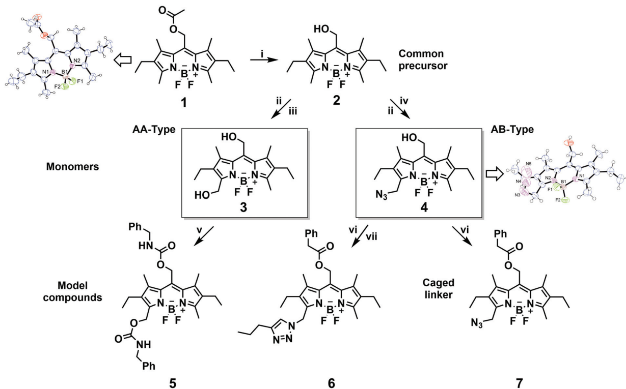
Scheme 1 Synthesis pathway towards bifunctional and hetero-bifunctional BODIPY monomers 3 and 4 and the synthesis of their respective small-molecular model compounds 5–7 . (i) NaOH, DCM/MeOH, H 2 O; (ii) NBS, DCM; (iii) H 2 O/DCM; (iv) NaN 3 , DCM/DMF; (v) benzyl isocyanate, toluene; (vi) phenylacetic acid, DCC, DMAP, DCM; (vii) pentynes, CuSO 4 ·5H 2 O, (+)-L-Na ascorbate, DCM/H 2 O.
