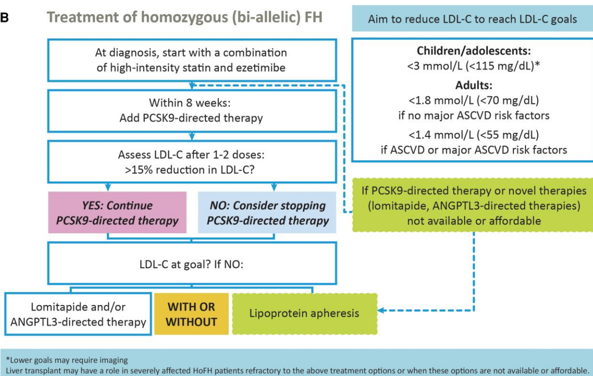
Figure 2 Identification and treatment of homozygous familial hypercholesterolaemia. (A) Algorithm for identification of phenotypic homozygous familial hypercholesterolaemia when clinically suspected in the absence of genetic data. (B) Treatment algorithm for homozygous familial hypercholesterolaemia (bi-allelic). ANGPTL3, angiopoietin-like 3; ASCVD, atherosclerotic cardiovascular disease; LALD, lysosomal acid lipase deficiency; LDL-C, low-density lipoprotein cholesterol; NGS, next-generation DNA sequencing; PCSK9, proprotein convertase subtilisin/kexin type 9.
