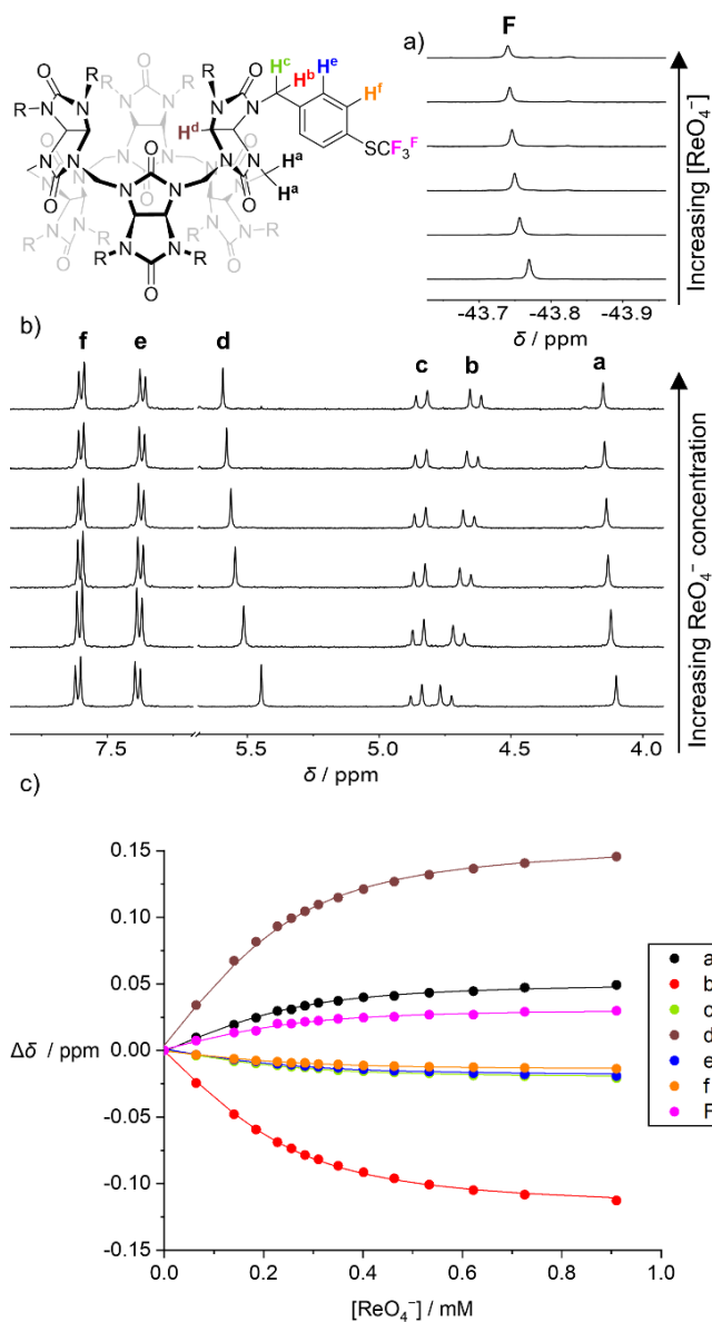
Figure 2. Titration of BU1 (0.24 mM) in the presence of the tetrabutylammonium (TBA) salt of CF 3 SO 3 - (11 mM) with a TBAREO 4 solution in CD 3 CN. a) Changes in the chemical shift of fluorine nuclei observed by 19 F NMR spectroscopy; b) changes in the chemical shifts of protons a-f observed by 1 H NMR spectroscopy; c) global fitting of the obtained data to a 1:1 model (Equation S7).
