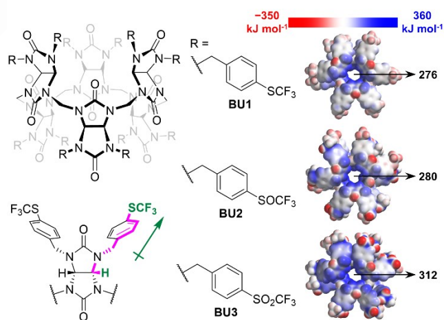
Figure 1. Structures of the bambusurils BU1-BU3 used in this work. The bonds through which the C-H bond is polarized by the electron-withdrawing groups are visualized on a single glycoluril unit in magenta colour. The calculated electrostatic potential maps show the electron deficient cavities (blue color) inside the macrocycles and the potential values inside the BU cavities are indicated. These calculations were performed in Spartan '18 1.4.4 after the structures were optimized with the semi-empirical PM6 method in vacuum.
