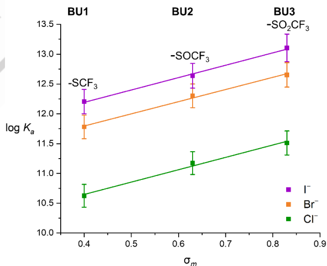
Figure 3. Hammett plot between the BU1 - BU3 bambusurils and halides in CD 3 CN. The slopes of the fitted lines are 2.04 (Cl - ), 2.07 (Br - ) and 2.08 (I - ).
