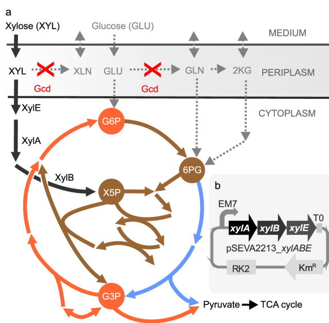
Fig. 1 | Pseudomonas putida EM42 PD310 used as a template strain in this study. Schematic illustration of (a) upper sugar metabolism of P. putida EM42 PD310 and (b) pSEVA2213_xylABE plasmid construct. The PD310 strain 18 capable of growth on D-xylose and its co-utilization with D-glucose bears low-copy-number plasmid pSEVA2213 with constitutive P EM7 promoter and a synthetic operon that encodes exogenous xylose isomerase pathway (XylA xylose isomerase and XylB xylulokinase) and xylose/H + symporter XylE from Escherichia coli BL21(DE3). The xylA and xylE genes are preceded by synthetic ribosome binding sites (RBS), while xylB was left with its native RBS. Note that the elements in the plasmid scheme are not drawn to scale. The PD310 strain was also deprived of the gcd gene, which encodes periplasmic glucose dehydrogenase (PP 1444 ) to prevent the transformation of xylose to the dead-end product xylonate (XLN). The exogenous pathway converts xylose to xylulose 5-phosphate (X5P), which enters the EDMP cycle formed by the reactions of the pentose phosphate pathway (brown arrows), the Embden-Meyerhof-Parnas pathway (orange arrows), and the Entner-Doudoroff pathway (blue arrows). Abbreviations: GLN, gluconate; G6P, glucose 6-phosphate; G3P, glyceraldehyde 3-phosphate; Km, kanamycin; 2KG, 2-ketogluconate; 6PG, 6-phosphogluconate; RK2, a broad-host-range origin of replication; TO, transcriptional terminator.
