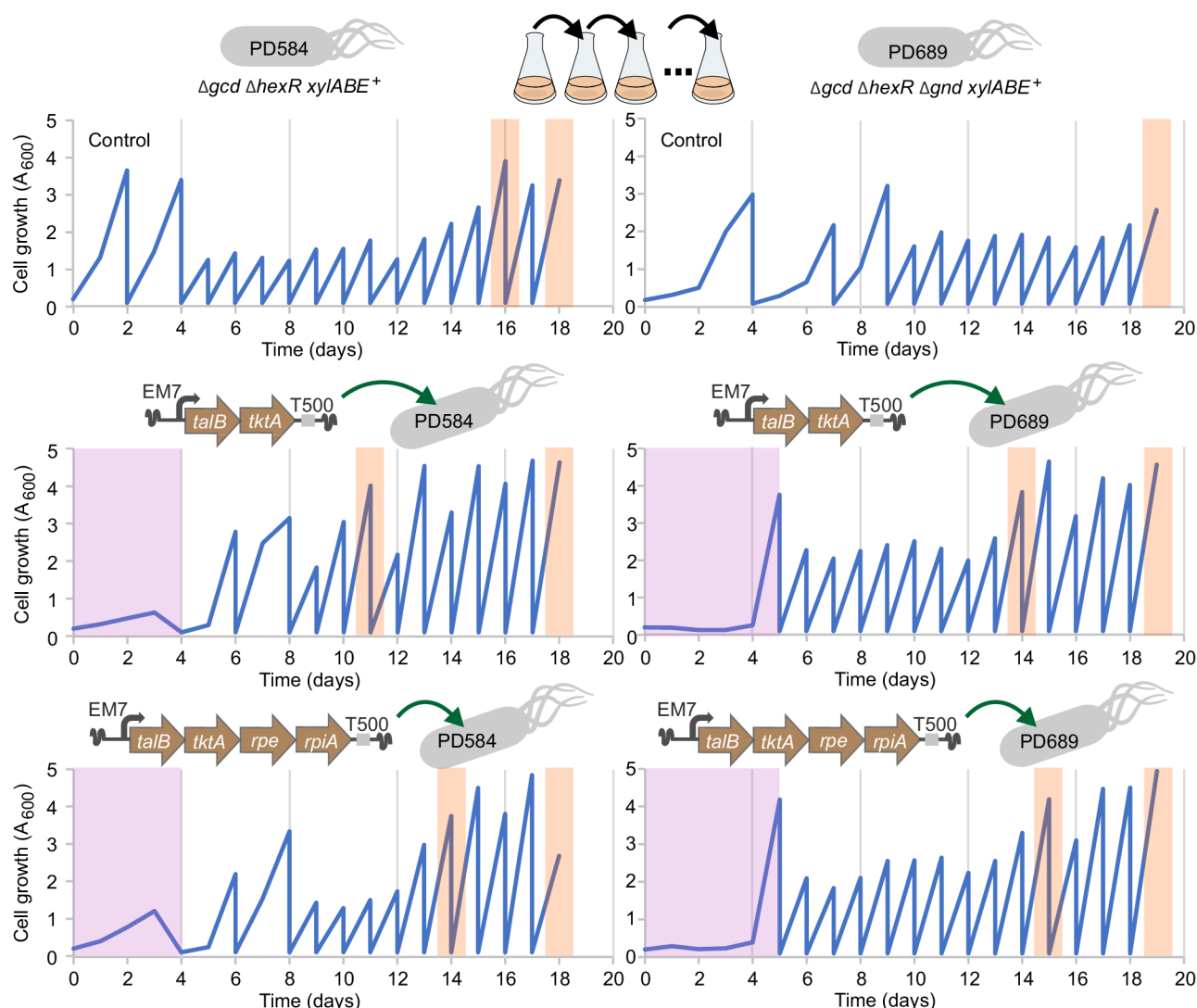
Fig. 5 | Adaptive laboratory evolution (ALE) on xylose of Pseudomonas putida PD584 and PD689 strains with and without integrated synthetic operons bearing pentose phosphate pathway (PPP) genes from Escherichia coli . Cells were cultured in 20 mL of M9 medium with 5 \text{ g L}^{-1} D-xylose and kanamycin and passaged in time intervals indicated in the graphs (upper two graphs depict ALE of PD584 and PD689 controls without implanted PPP genes and the lower four graphs depict ALE of PD584 and PD689 transformants after insertion of pBAMD1-4 plasmid constructs with PPP genes). The initial period where PD584 and PD689 transformants were cultured in M9 medium with xylose and two antibiotics (kanamycin, streptomycin) to select for the integration of tktA-talB and tktA-talB-rpe-rpiA cassettes is indicated by pink shading. ALE of cultures in M9 medium with xylose and
