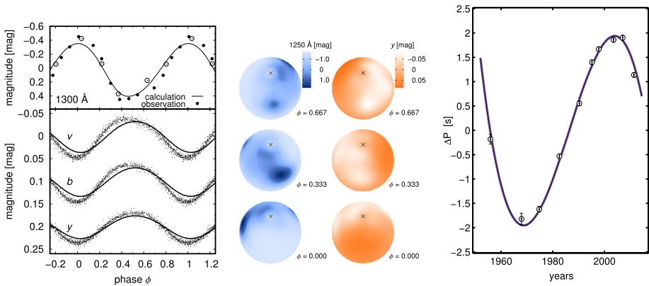
Fig. 1 Variability of chemically peculiar CU Vir. Left: The light curve in ultraviolet (upper panel) and visual (lower panel – Strömgren vby filters) domains. Empty circles denote HST observations (Krtićka et al. 2019). Middle: The emergent intensity at various rotational phases \phi in the ultraviolet (blue plots) and visual (orange plots) domains. Right: Rotational period variations with respect to the mean period derived from photometry (Mikulášek et al. 2011).
