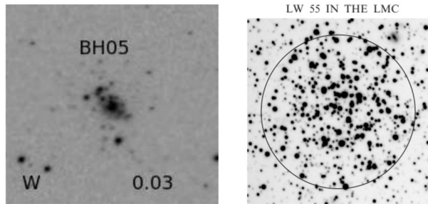
Fig. 4 Extra-galactic clusters in Andromeda Galaxy (left) and in the Large Magellanic Cloud (right). Images were taken from Caldwell et al. (2009) and Kaluzny and Rucinski (2003).
