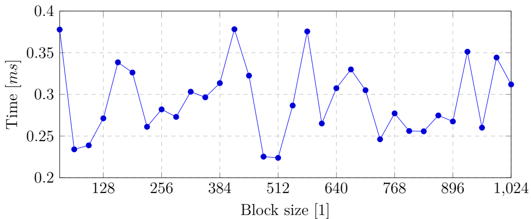
Figure 5.1: Block size
