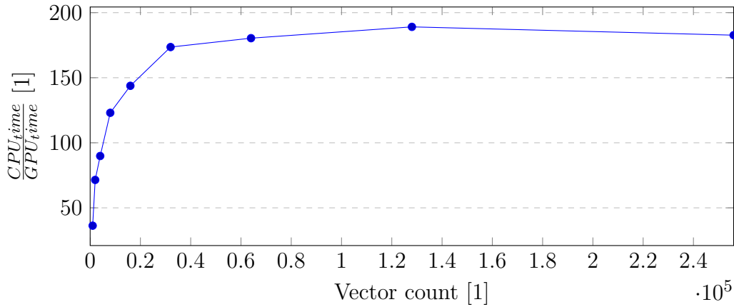
Figure 5.3: Overall speed-up
