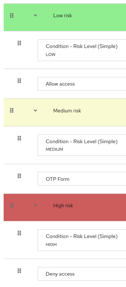
Figure 6.18: Simple Risk Level Flow.
