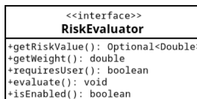
Figure 6.9: Risk Evaluator Diagram.
