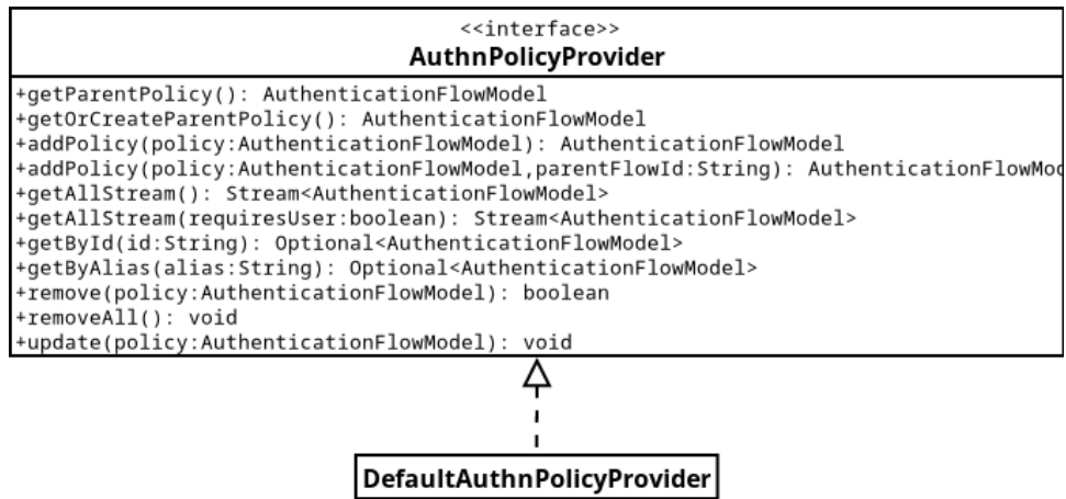
Figure 7.2: Authentication Policy Provider.
