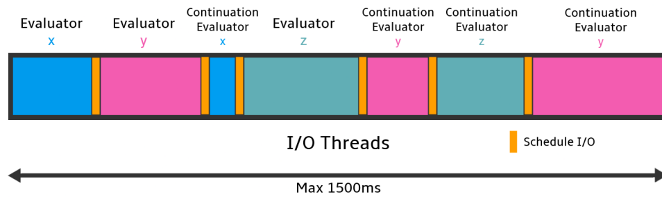
Figure 7.13: I/O Threads.
