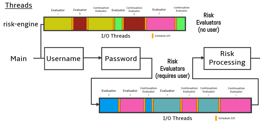
Figure 7.14: Asynchronous Processing Flow.
