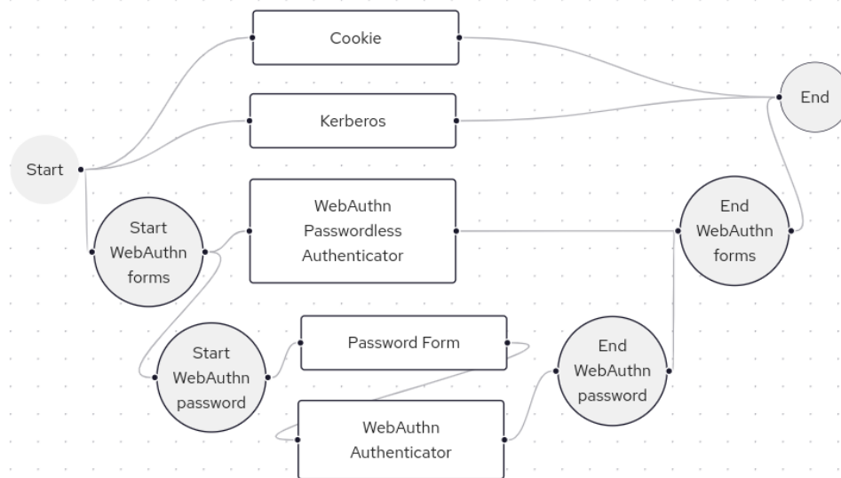
Figure 4.1: WebAuthn Flow.
