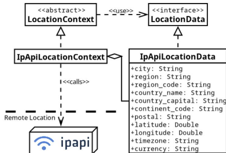
Figure 7.23: External Service ipapi .
