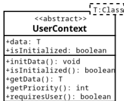
Figure 6.1: User Context Diagram.
