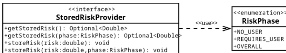
Figure 6.13: Stored Risk Provider Diagram.
