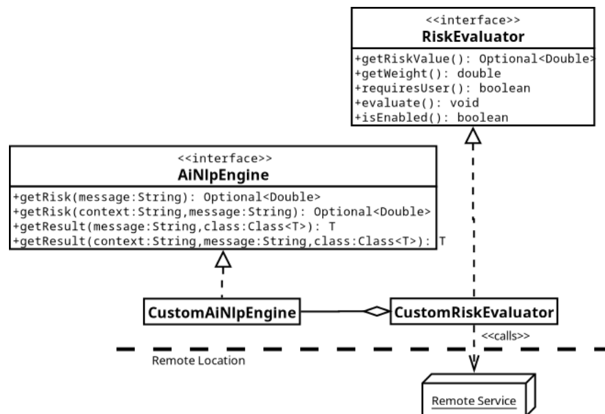
Figure 6.20: Risk Evaluator and AI NLP Engine Diagram.
