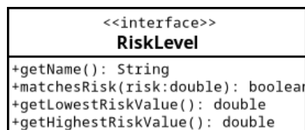
Figure 6.15: Risk Level Diagram.
