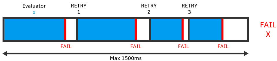
Figure 7.15: Risk Evaluators Retry Mechanism.
