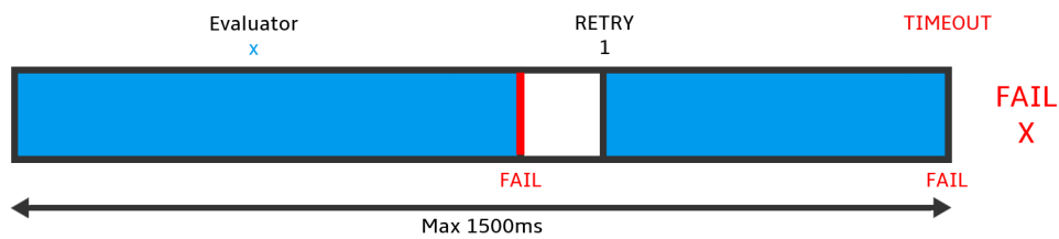
Figure 7.16: Risk Evaluators Timeout.
