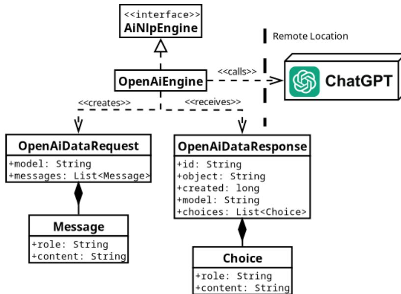
Figure 7.18: OpenAI Integration.
