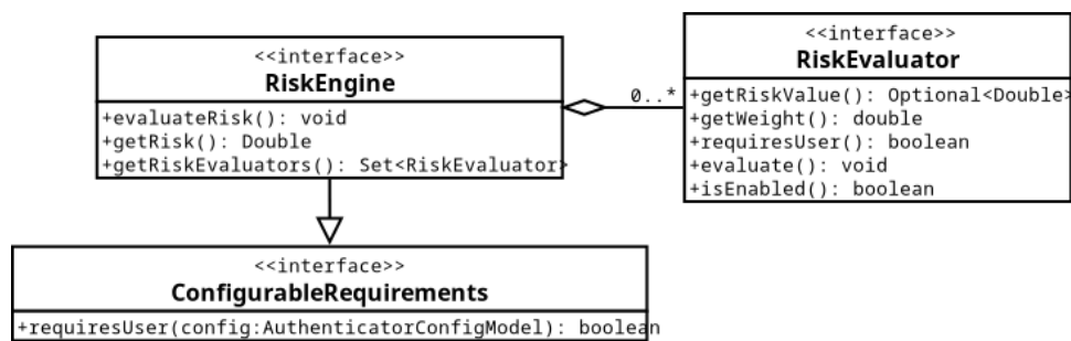
Figure 6.11: Risk Engine Diagram.
