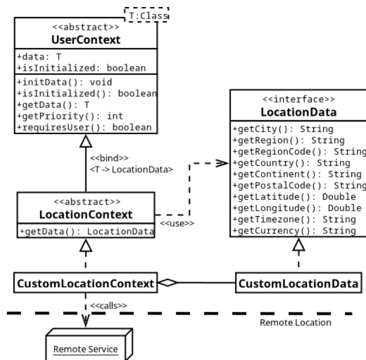
Figure 6.21: Remote Location Context.
