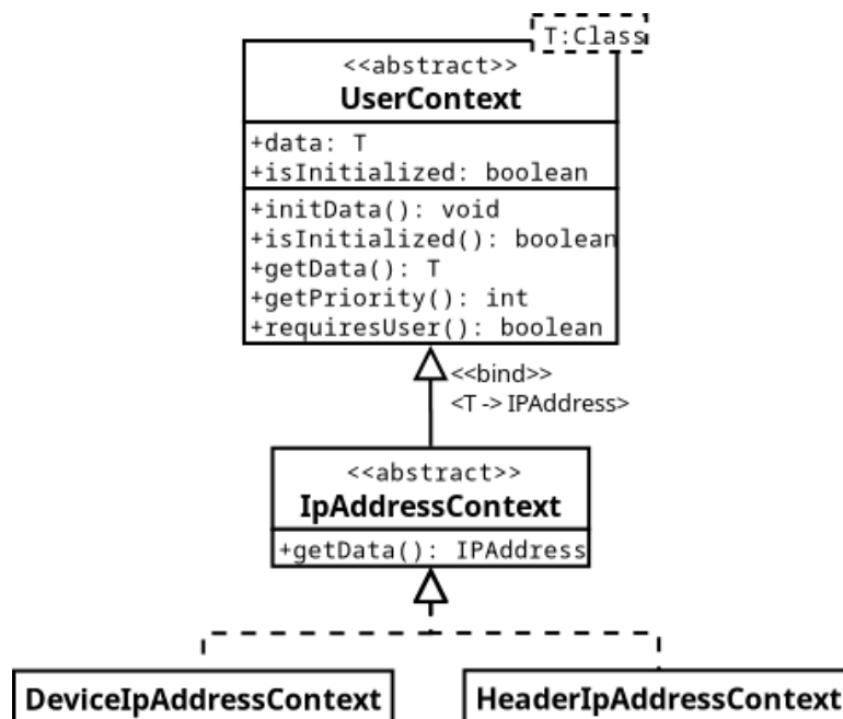
Figure 6.2: IP Address User Context Diagram.
