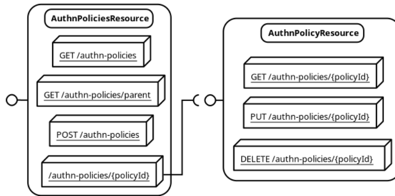
Figure 7.6: Authentication Policies REST API.
