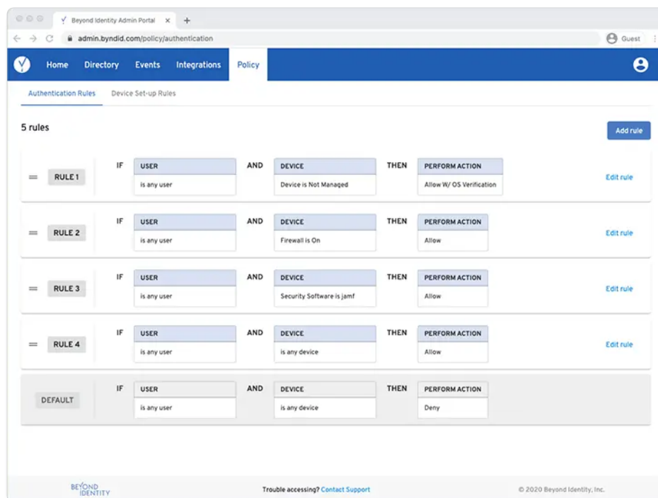
Figure 3.3: Beyond Identity Authentication Policies. Source: [26].
