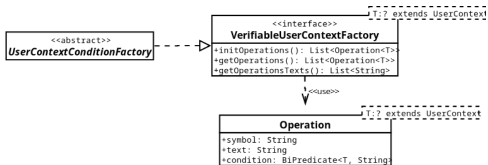
Figure 6.3: User Context Condition Diagram.
